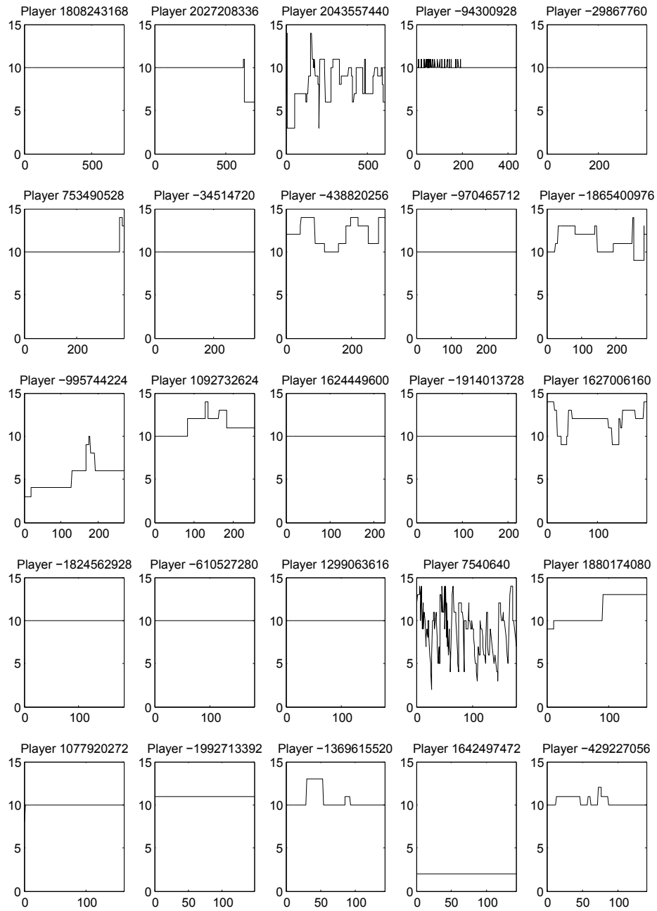
Figure 6: Change in game level ( y -axis) over games played ( x -axis) for individual players.
