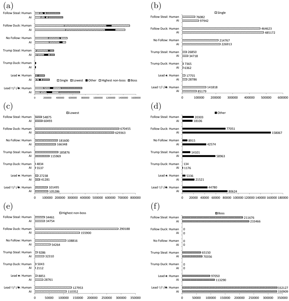
Figure 7: Comparison of human and AI usage of abstract moves: (a) shows the total number of moves played per category, (b)–(f) show, within each category, how frequently the player or AI plays their (b) only, (c) lowest, (e) highest non-boss, (f) boss or (d) any other card in that category.
