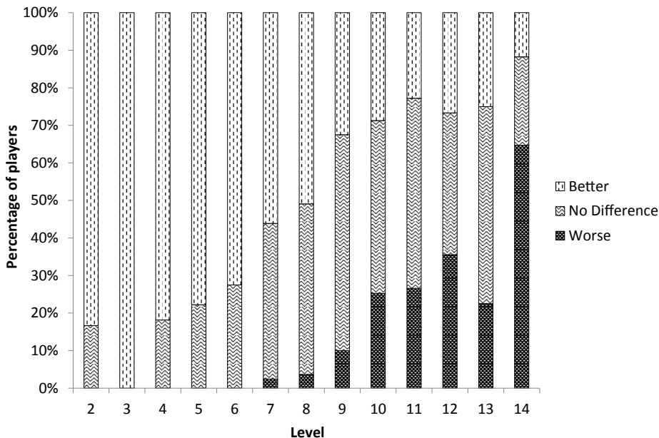
Figure 4: Comparison of player performance at each AI level, classifying players based on confidence intervals on their win rates. Each bar shows the number of players classified as better than, no different from and worse than the AI opponents at that level, as a proportion of the number of players with at least one game at this level (see Figure 2).
