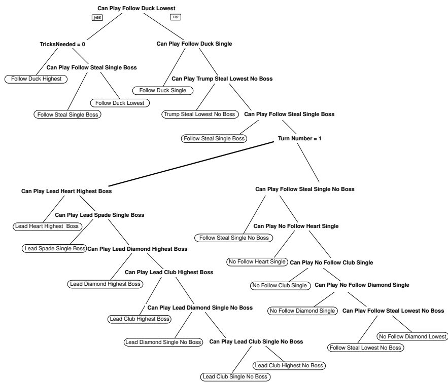
Figure 8: Model of average Human Strategy.
